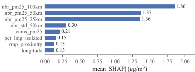
(b) top 8 of 38 features
